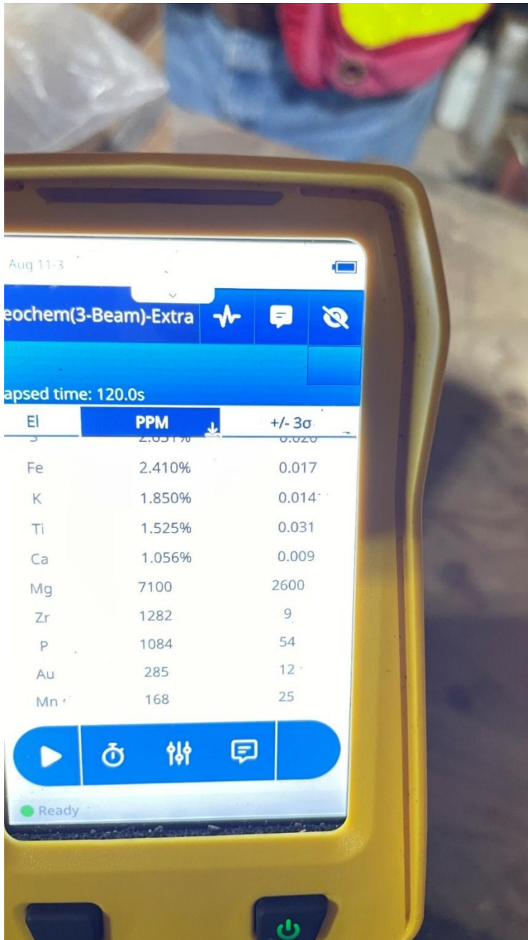
Photo 2: Confirmation of Gold by Portable XRF. Note the result of 285 ppm Au is Equal to 285 gram/tonne gold. A single occurrence of visible gold while significant does not indicate the average assay grade of the yet to be received sample width.
