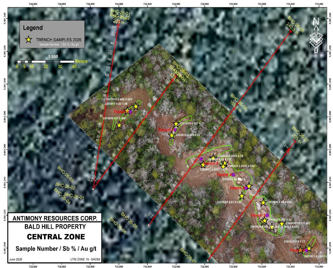
Figure 2: Trench Locations at Central Zone. Note location of Proposed drill holes in first round of drilling. ATMY trenching outlines are in green. Samples collected are represented by gold stars
