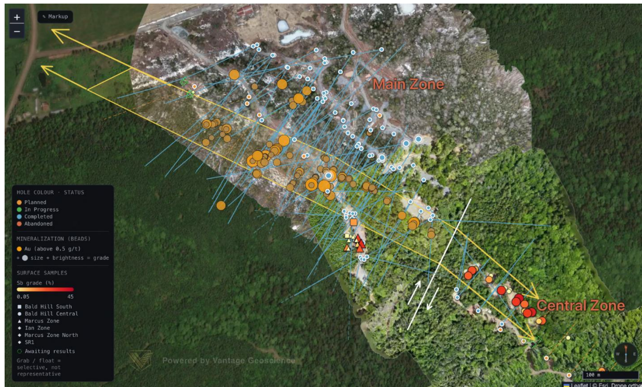
Figure 1: Surface Trace of the Main Zone at Bald Hill Showing Values of Gold Projected to Surface. Note a subsidiary zone to the Northeast. This is a splay also defined by antimony results.
